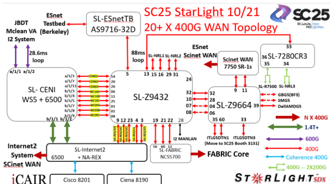
Topology of SDX Interconnections for SC25 at the StarLight International/National Communications Exchange Facility
